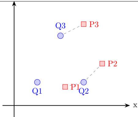
Iteration 1 - Data Association (Pairing Source P with Nearest Target Q)
